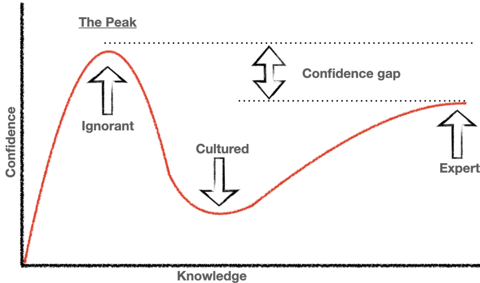
Dunning-Kruger Effect
